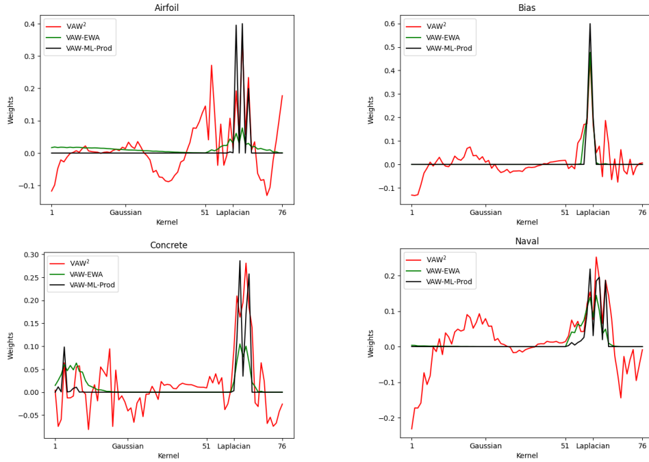
FIG. 2. Terminal weights of \text{VAW}^2 , VAW-EWA and VAW-ML-Prod algorithms.
