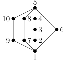
FIG. 1. Hasse diagram of a 5-partite poset.
