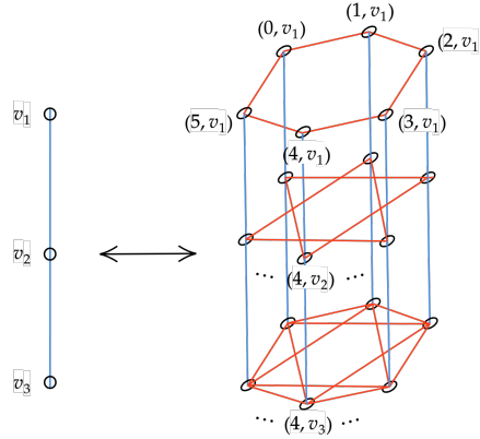
FIG. 1. From left to right: a path graph H on 3 vertices and the corresponding sandwich graph G with m = 3 layers. From top to bottom, the layers are circulant graphs: G_1 = C_6(1) , G_2 = C_6(2) , and G_3 = C_6(1, 2) .
